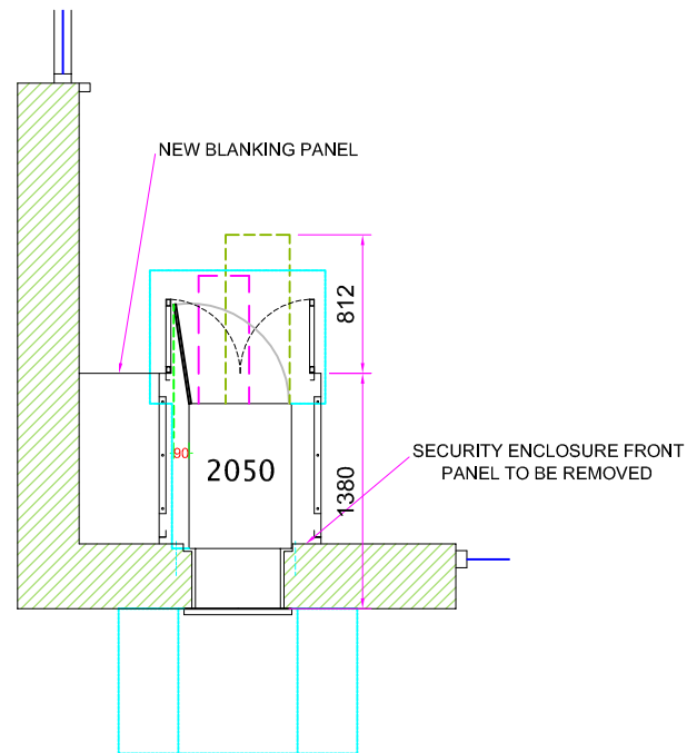
PROPOSED (PART) PLAN
