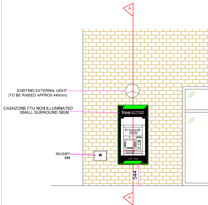
PROPOSED ELEVATION
