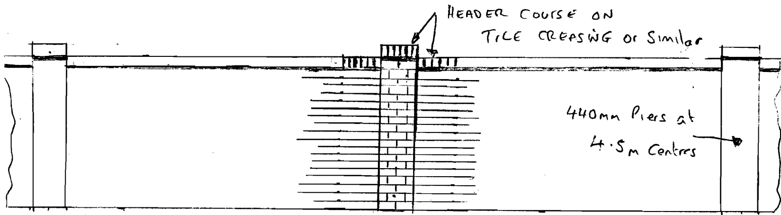
Part elevation SCALE 1:50
