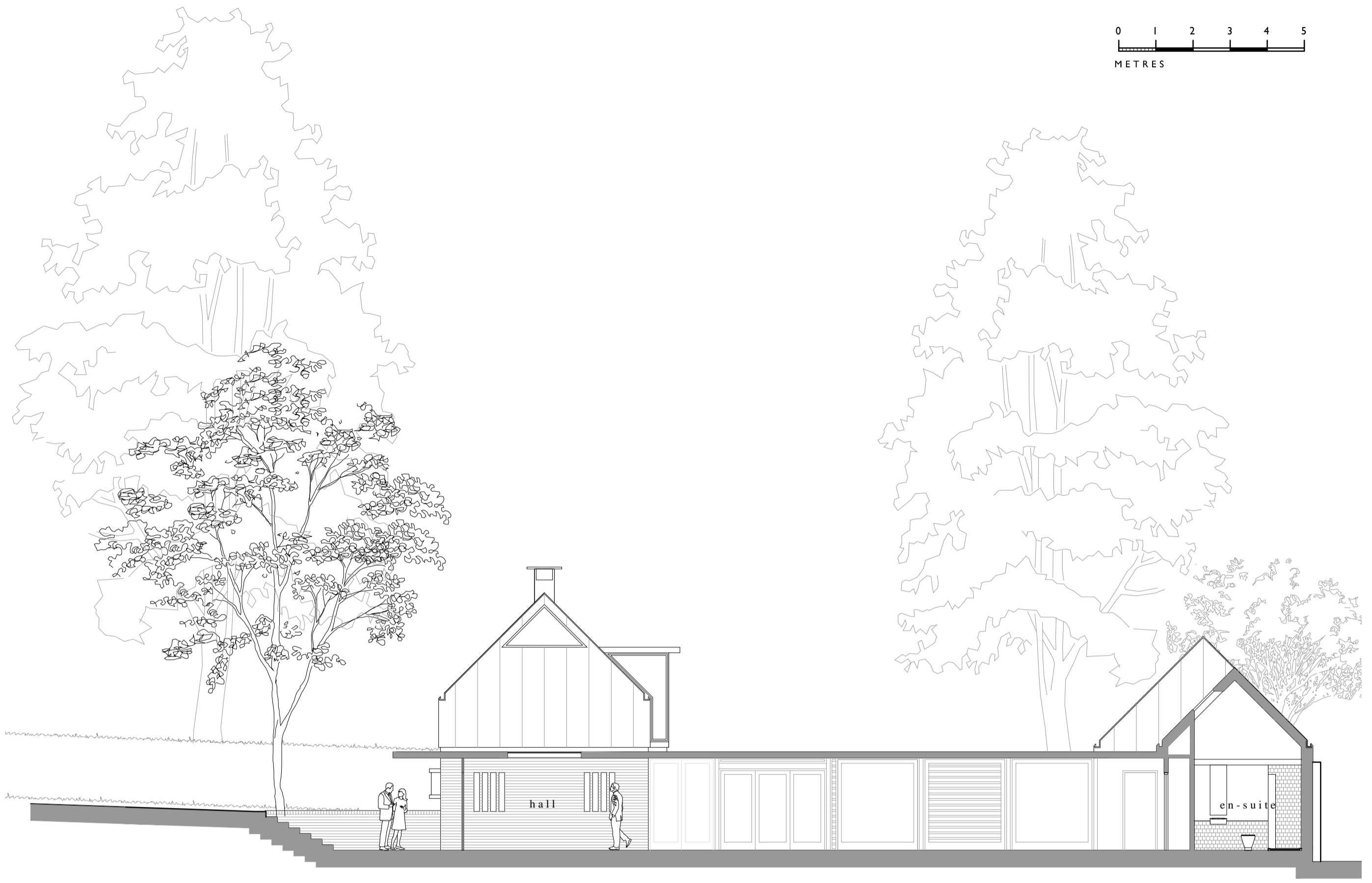
SECTION C-C
