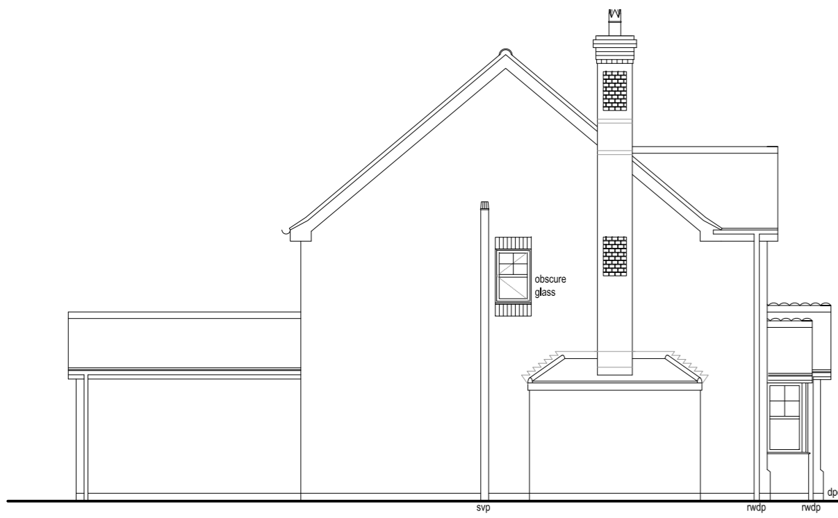
SIDE ELEVATION
