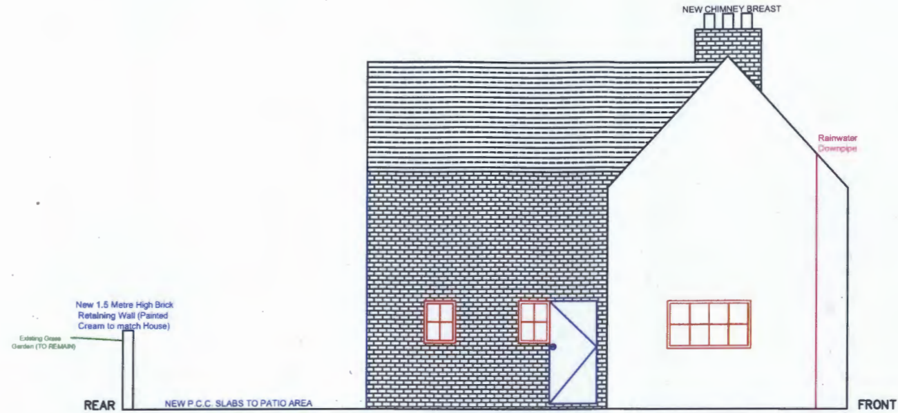
Proposed Side Elevation (North Facing)
