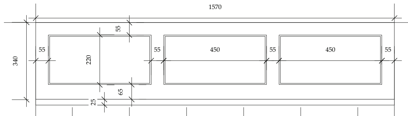
Window W2 External Elevation 1:10
