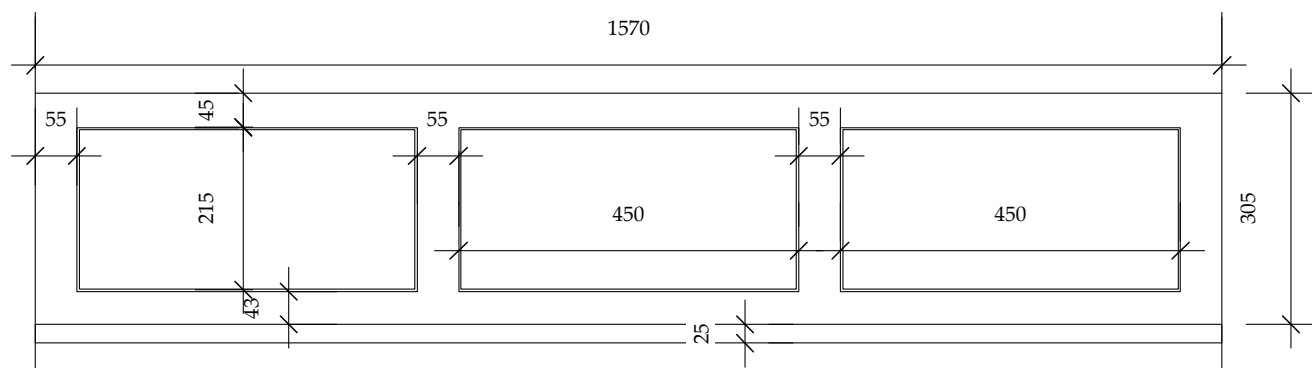
Window W2 Internal Elevation 1:10
