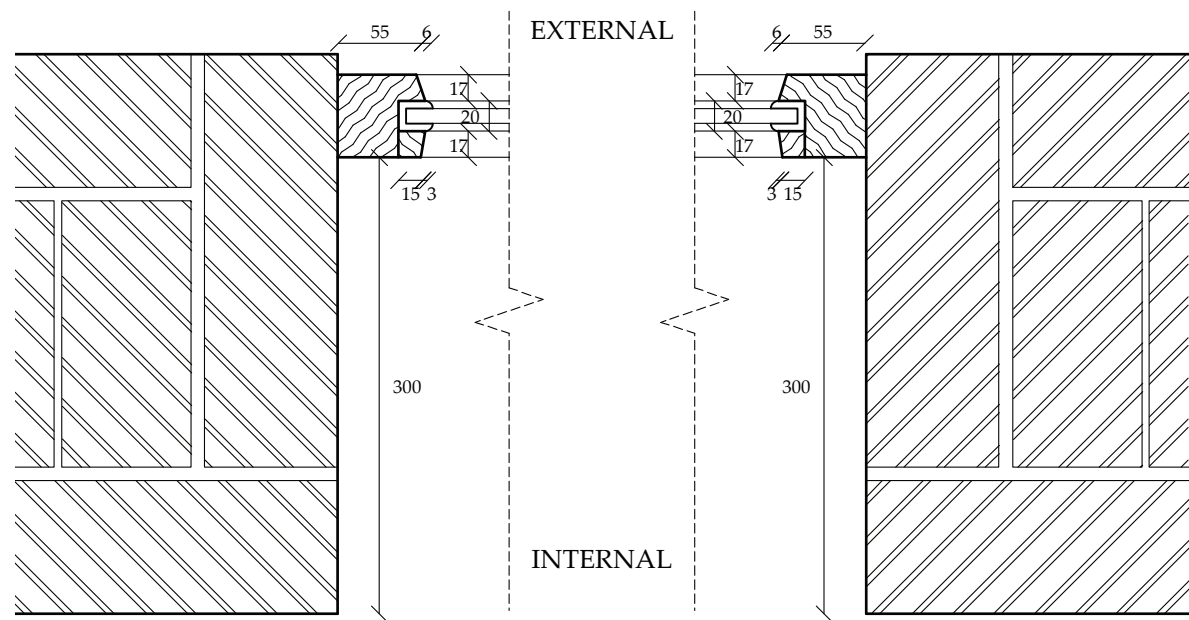
Window W2 Plan Detail 1:10
