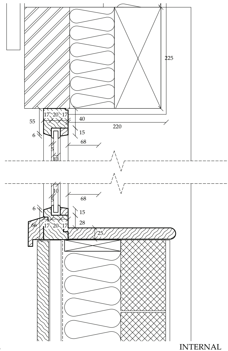
Window W2 Detail 1:5
