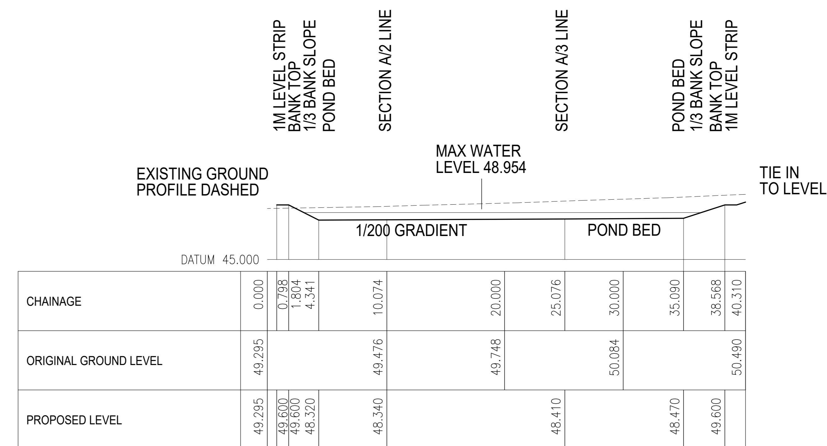
Section A/1 along Basin A
