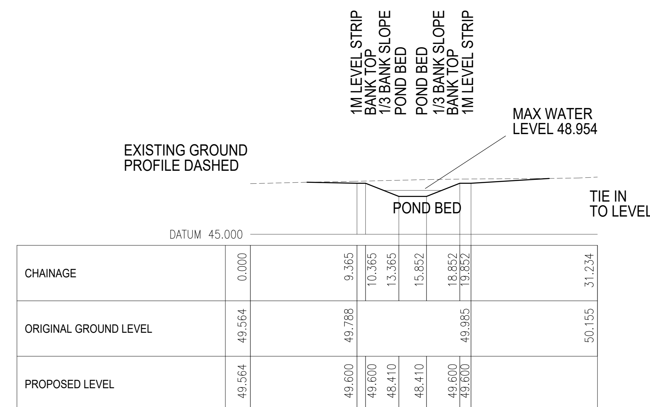
Section A/3 along Basin A
