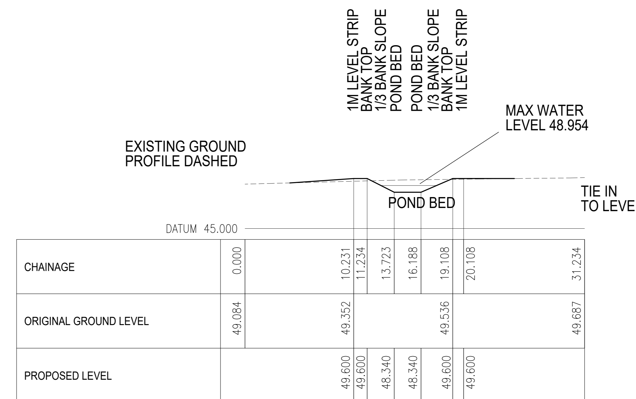
Section A/2 along Basin A
