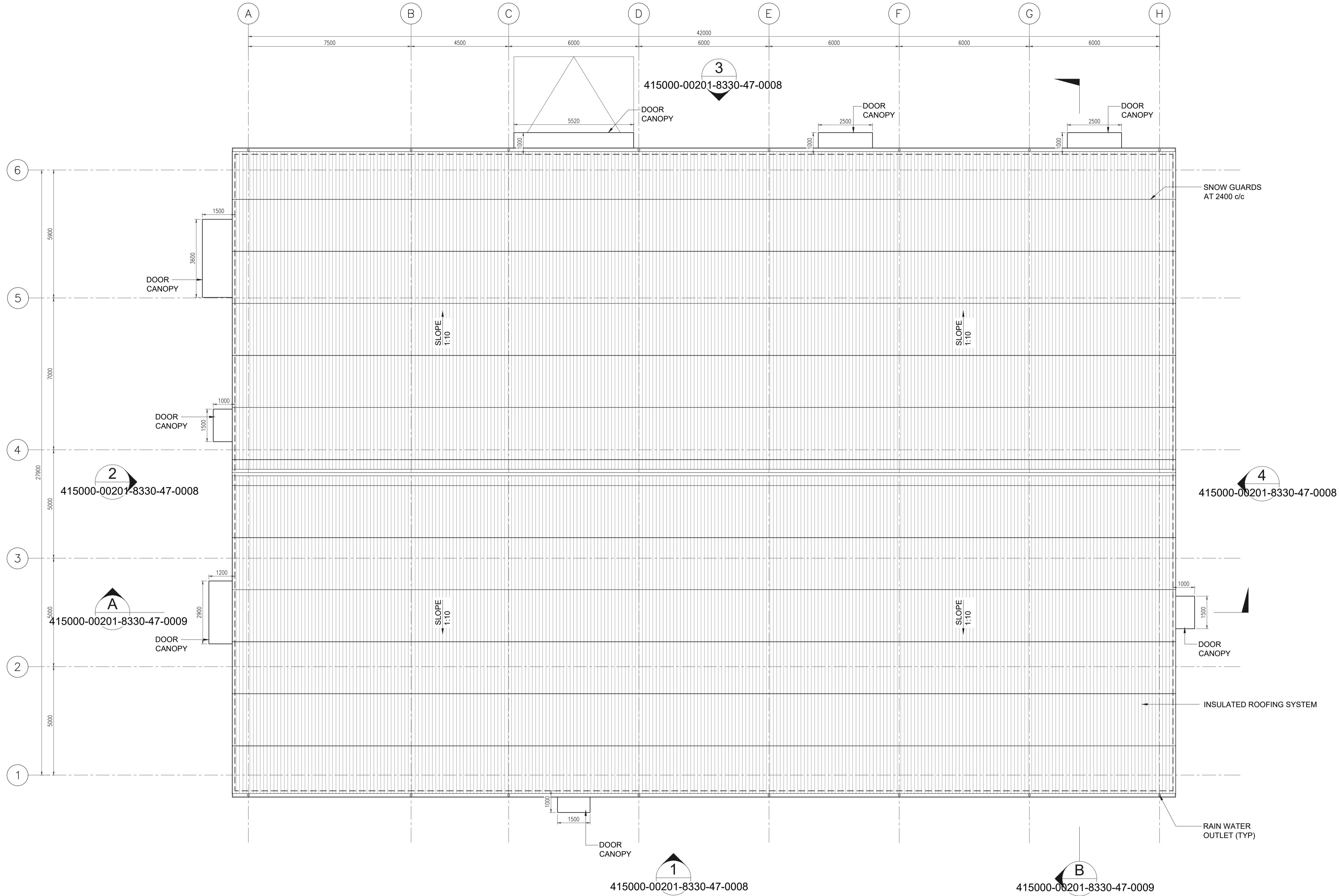
ROOF LEVEL PLAN SCALE - 1:100
