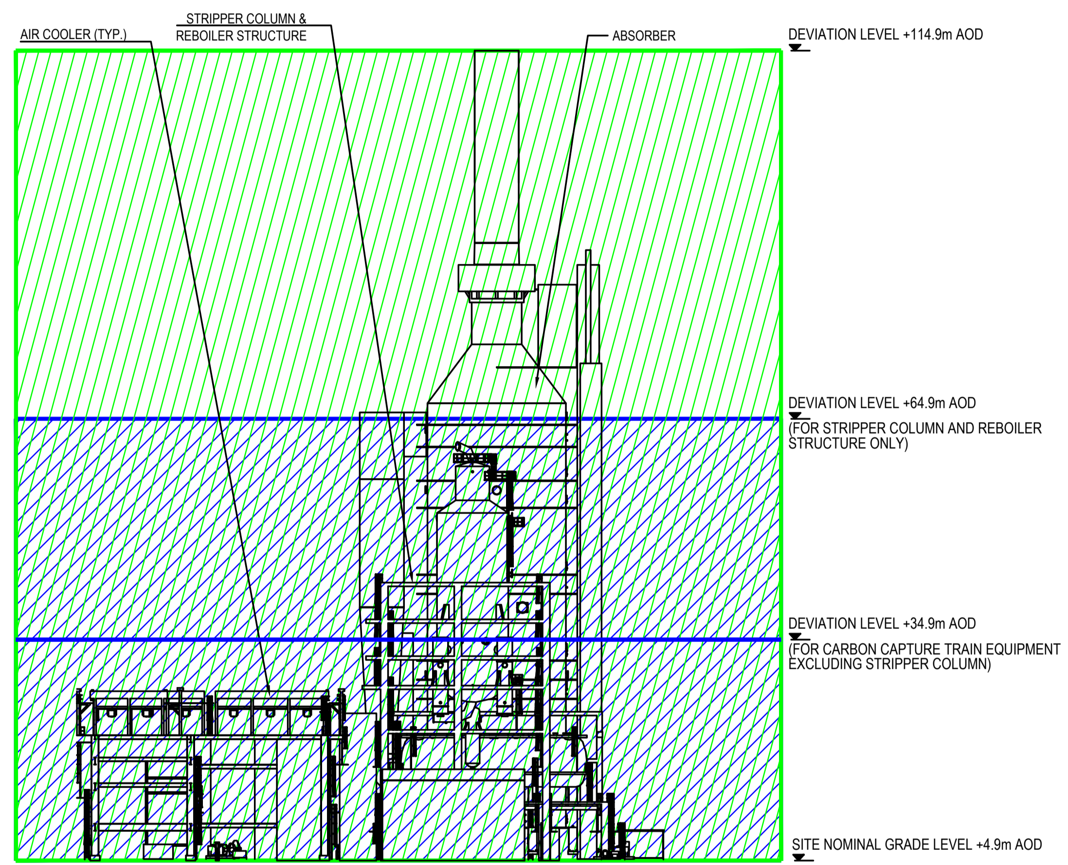
SECTION LOOKING WEST ON 'P-P'
