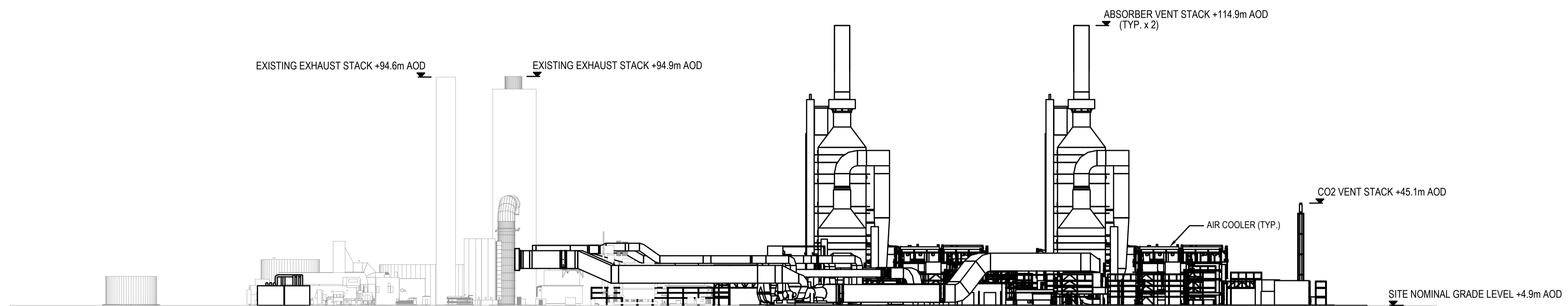
ELEVATION LOOKING EAST ON 'B-B'
