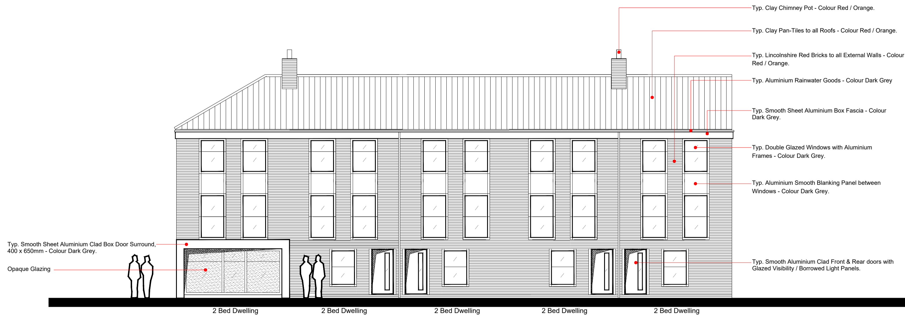
Proposed Indicative Front Elevations - Plots 01 to 05.
