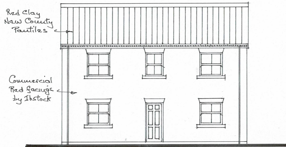
NORTH ELEVATION
