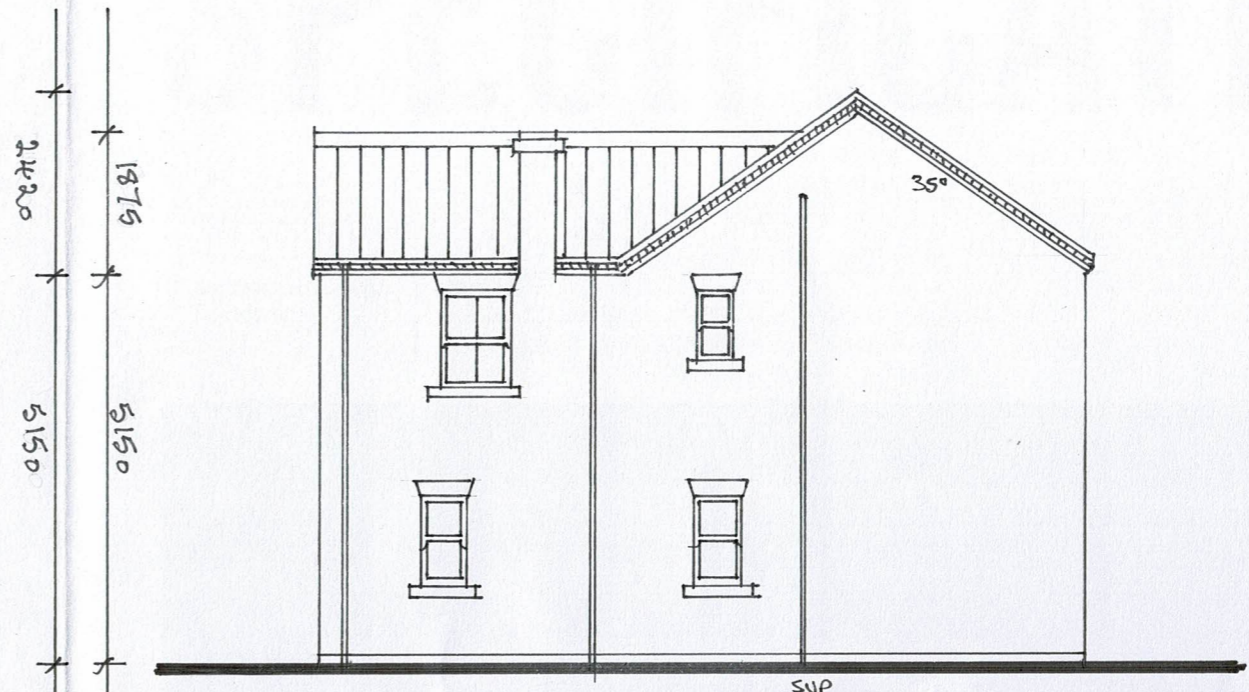
EAST ELEVATION.
