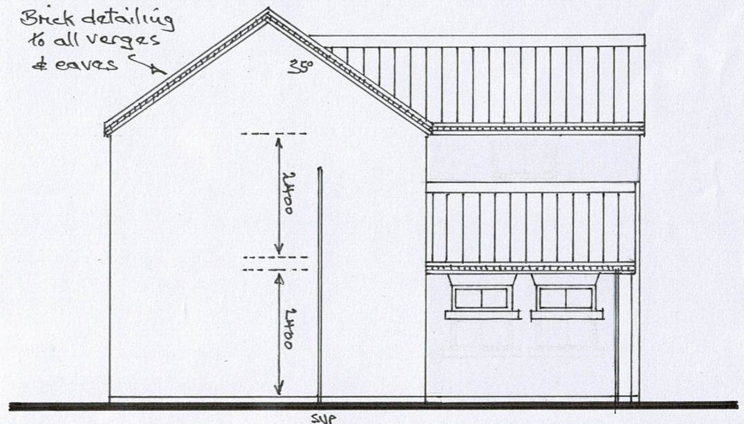
WEST ELEVATION
