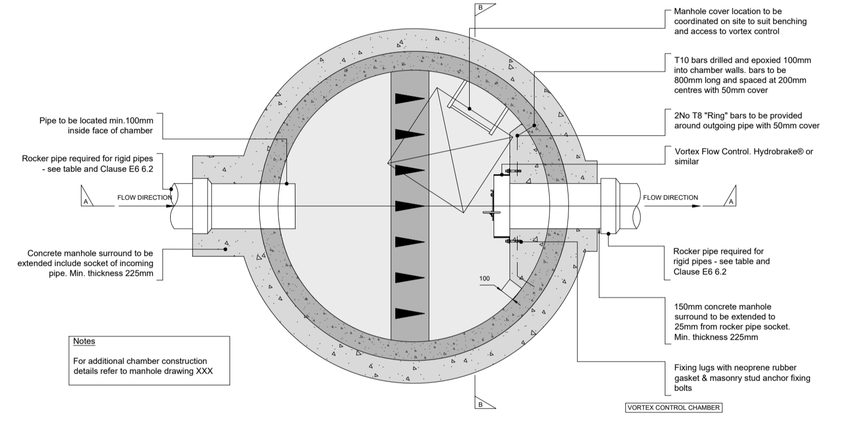
TYPICAL VORTEX CONTROL CHAMBER (SCALE 1:20)
