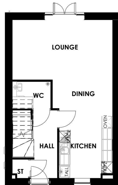
GROUND FLOOR PLANNING 1 : 100
