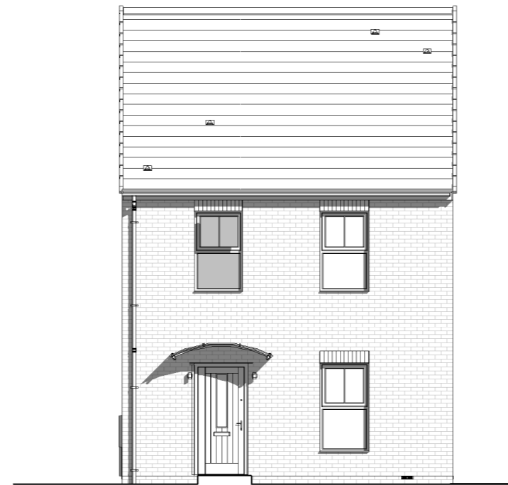
FRONT ELEVATION 1 : 100
