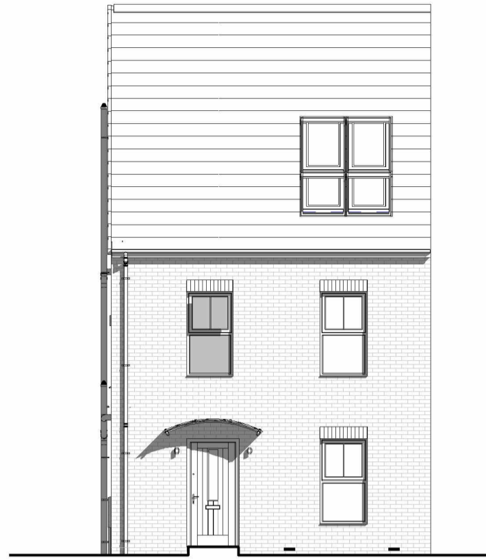
FRONT ELEVATION 1 : 100
