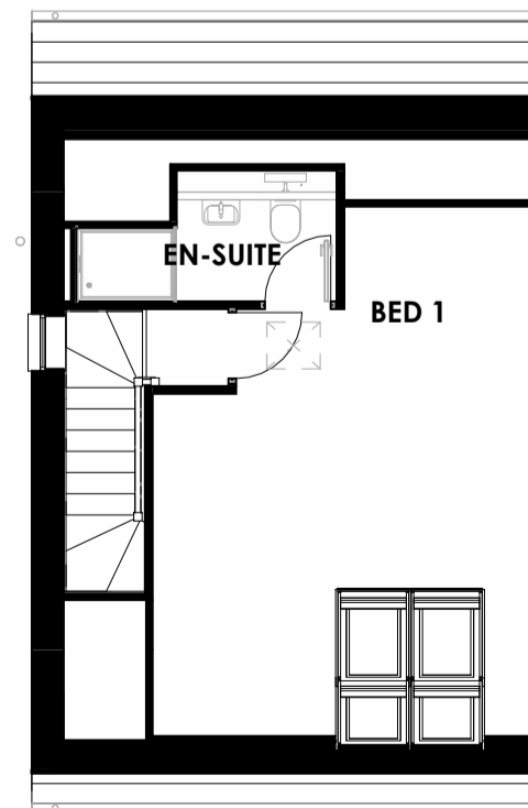
SECOND FLOOR PLANNING 1 : 100
