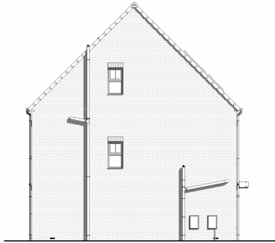
LEFT ELEVATION 1 : 100
