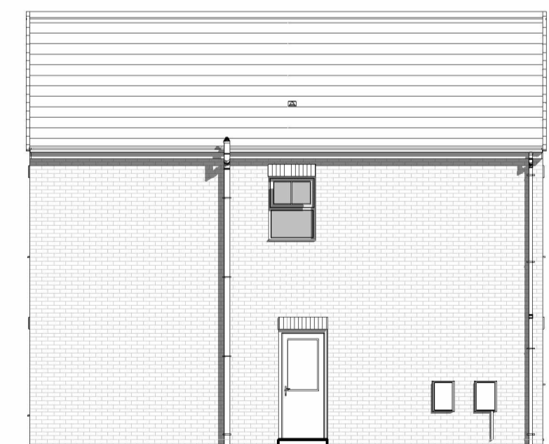
REAR ELEVATION 1 : 100
