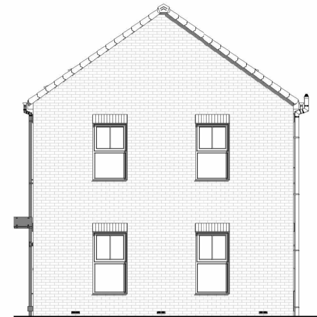
SIDE ELEVATION 1 : 100
