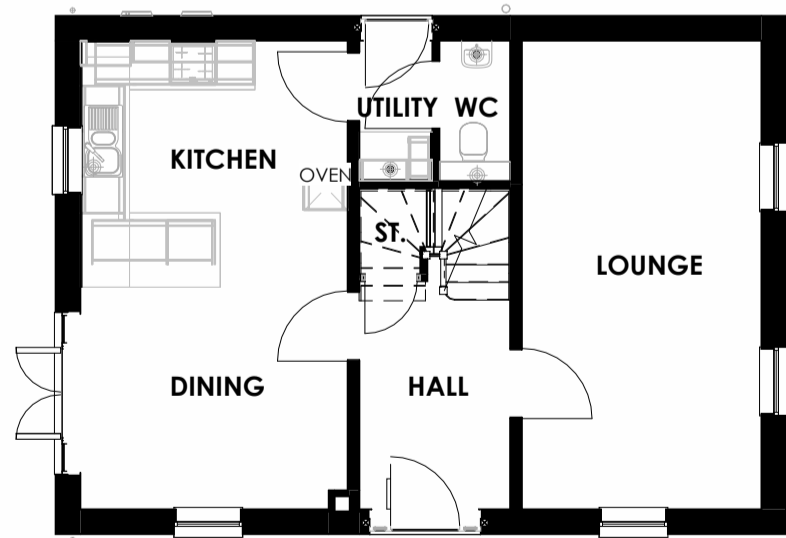
GROUND FLOOR PLANNING 1 : 100
