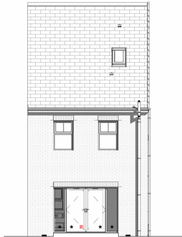
REAR ELEVATION 1 : 100
