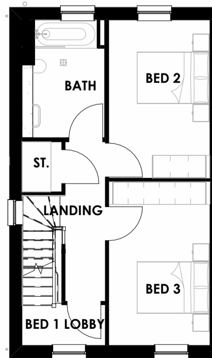
FIRST FLOOR LAYOUT 1 : 100
