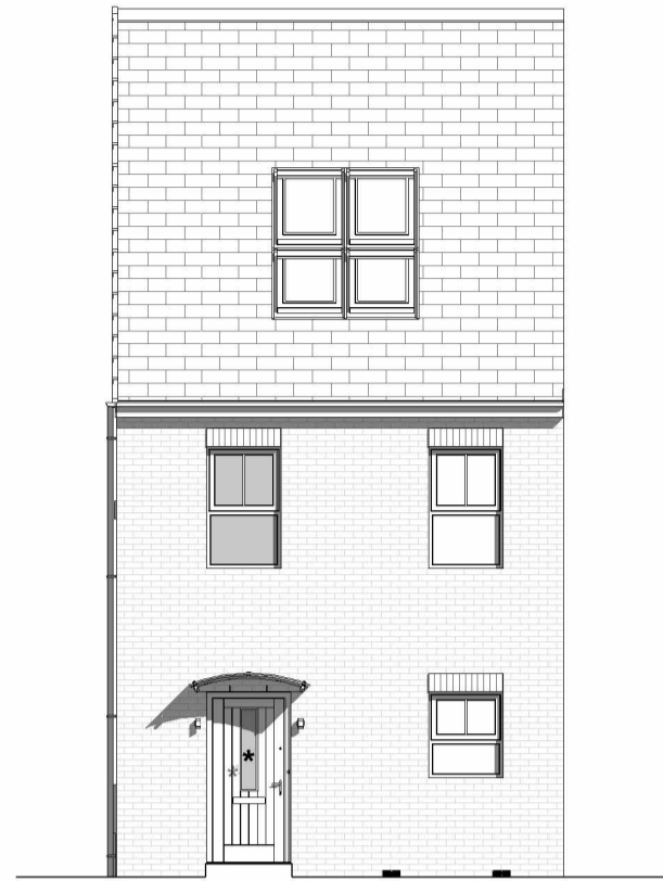
FRONT ELEVATION 1 : 100
