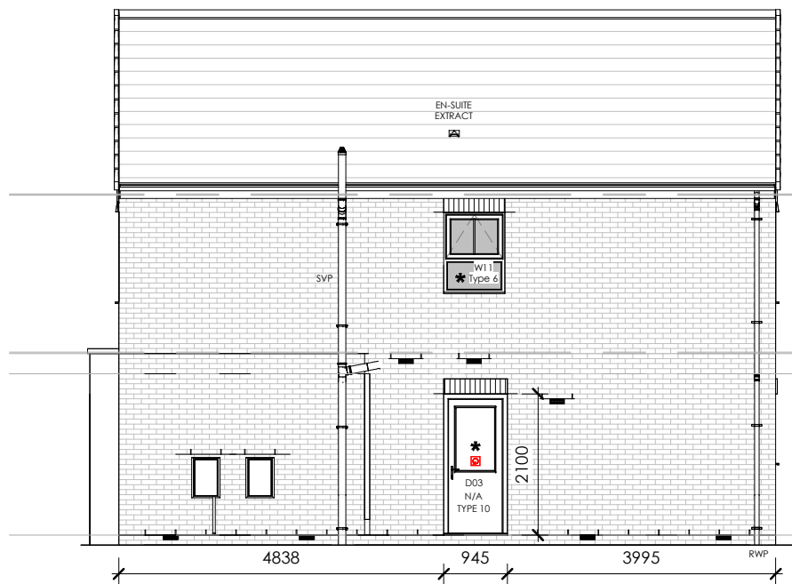
WELCOME CENTRE ELEVATION C
