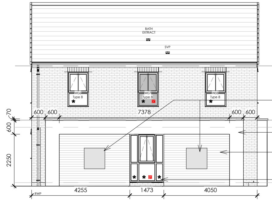
WELCOME CENTRE ELEVATION A
