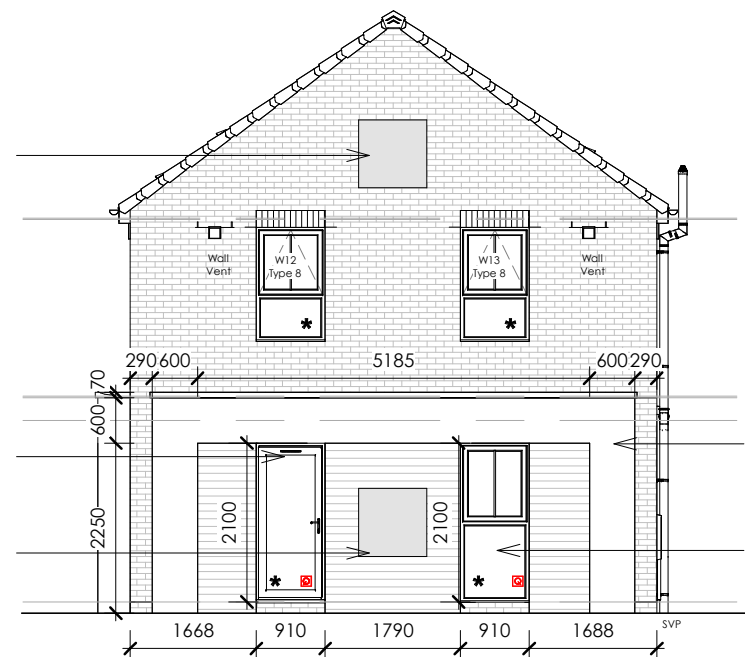
WELCOME CENTRE ELEVATION D
