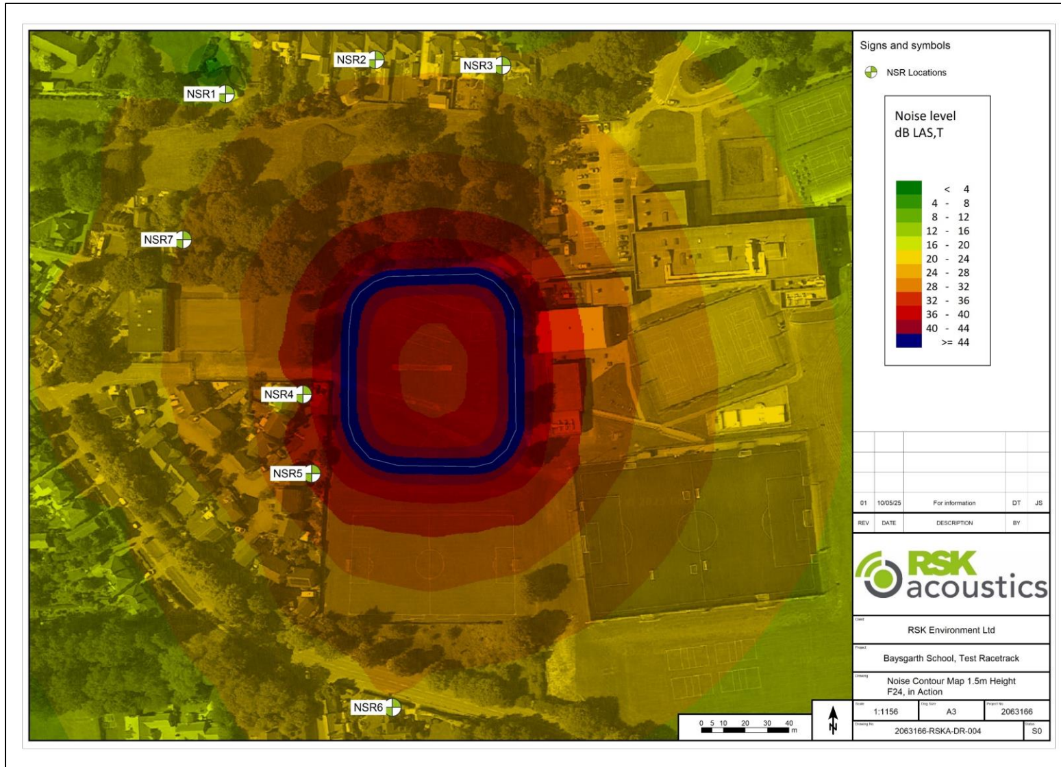
Figure G-2 Noise Contour Map @ 1.5 m, Daytime (07:00-23:00) – F24, In Action
