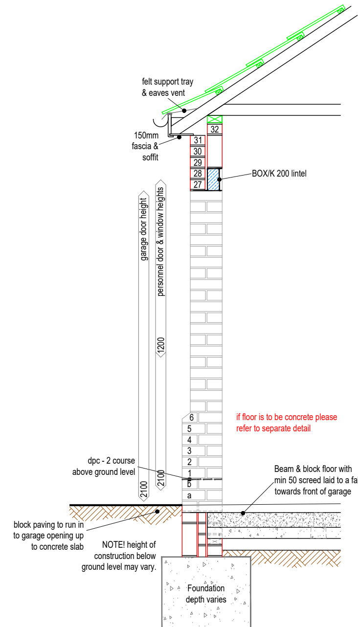
TYPICAL SECTION 1/25
