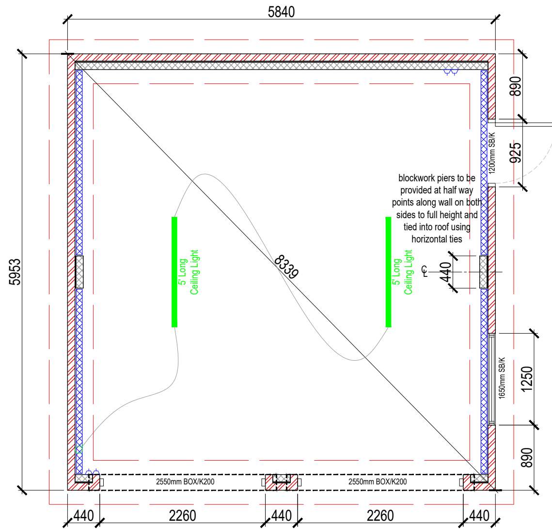
FLOOR PLAN 1/50
