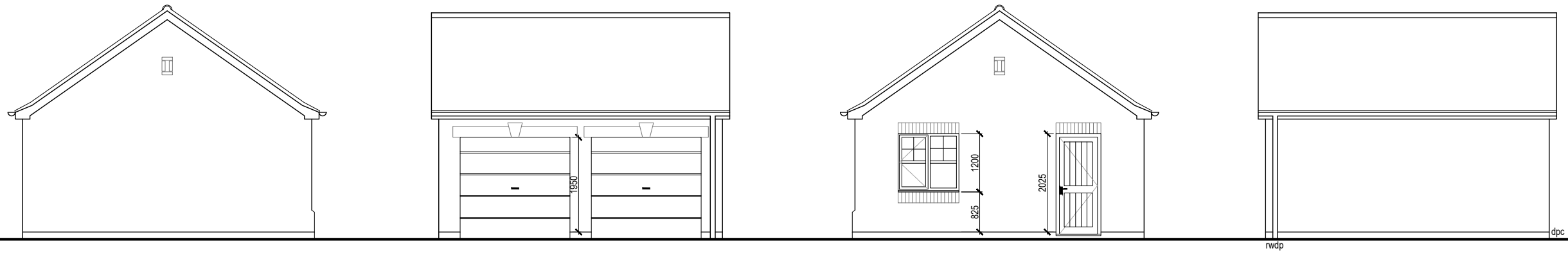
ELEVATIONS 1/100
