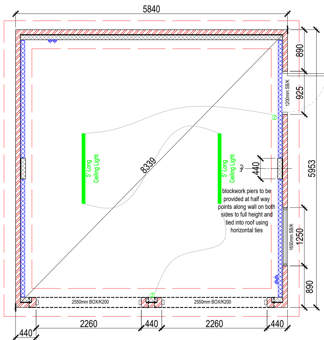
FLOOR PLAN 1/50
