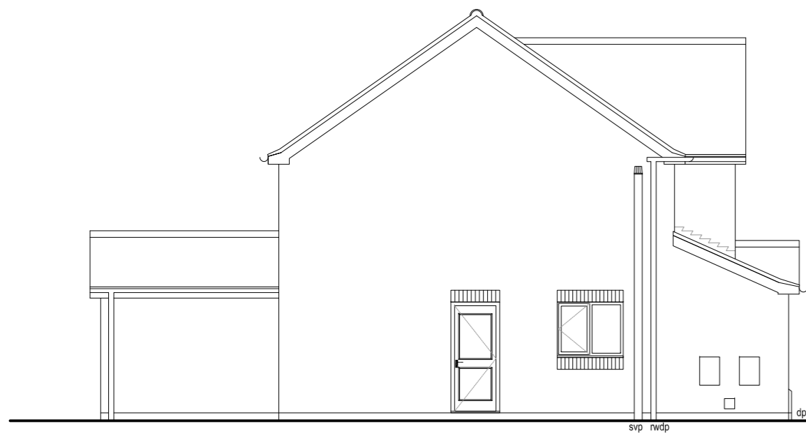
SIDE ELEVATION
