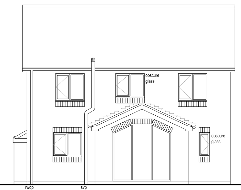
REAR ELEVATION
