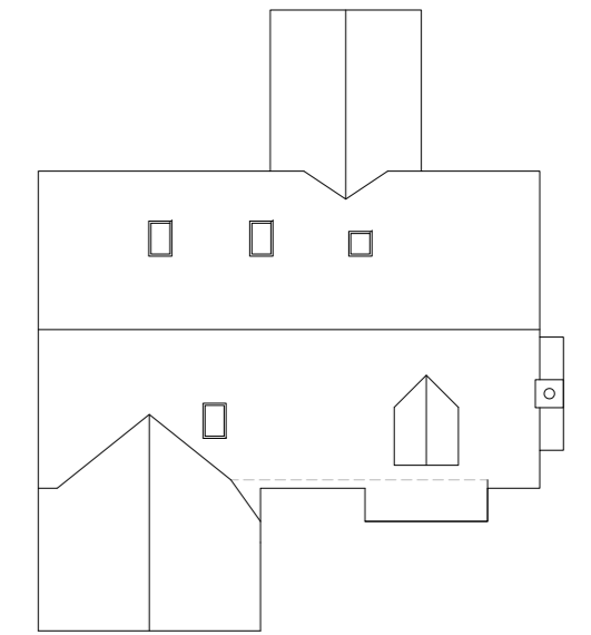
ROOF PLAN
