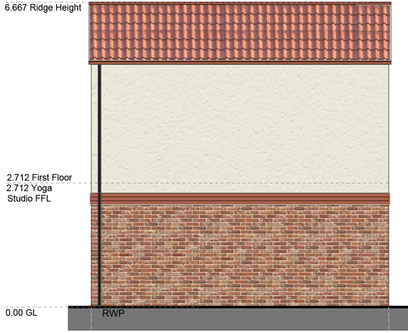
6515 Proposed Boundary Elevation - Scale - 1:50
