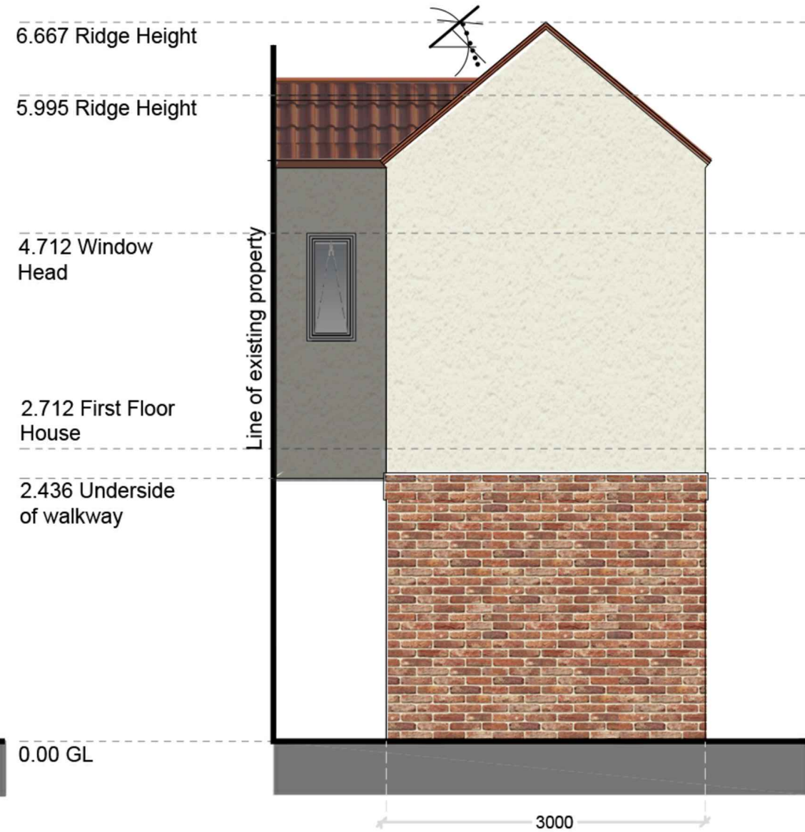
Proposed Leading Elevation - Scale - 1:50
