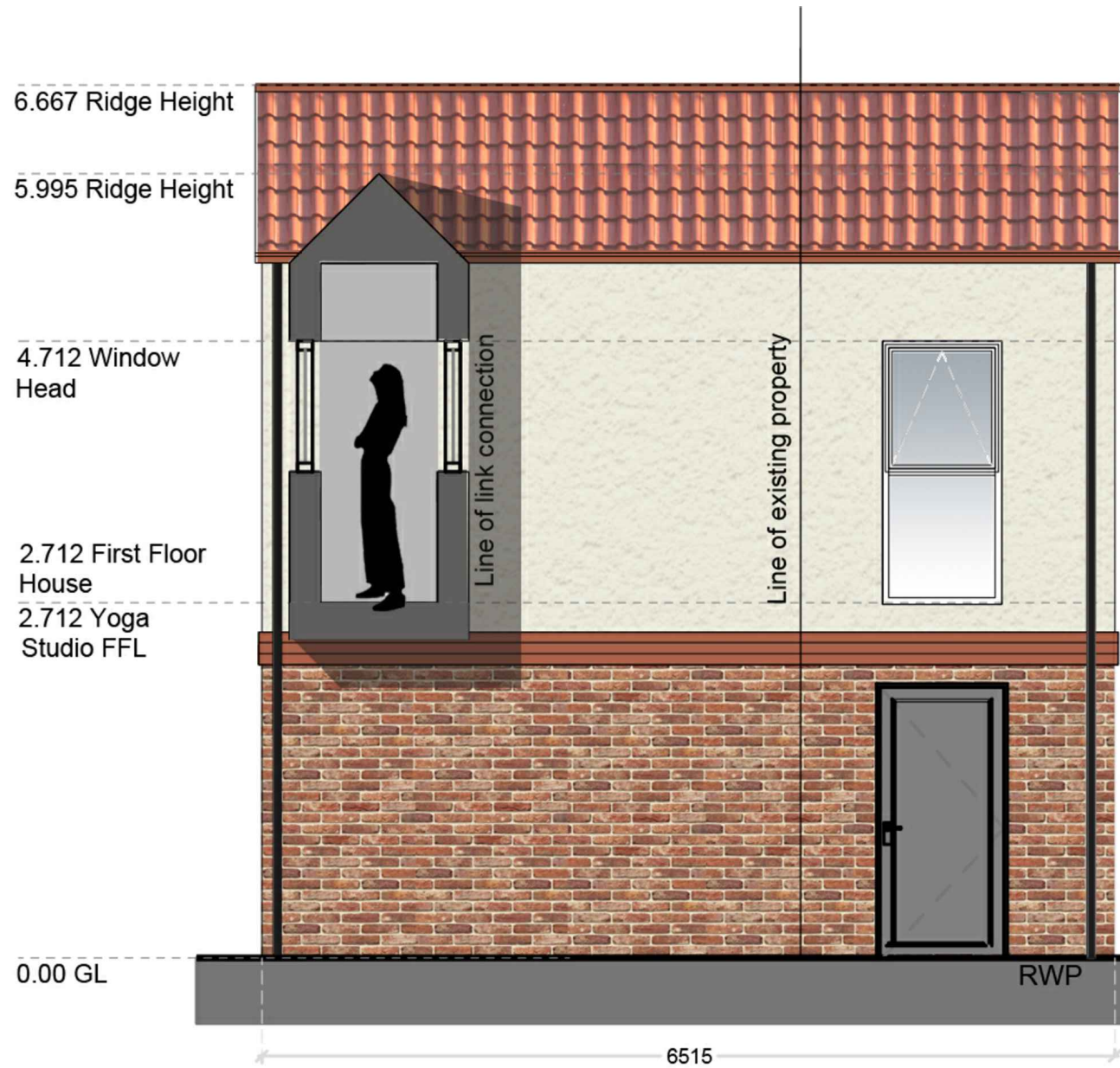
Proposed Internal walkway Elevation - Scale - 1:50
