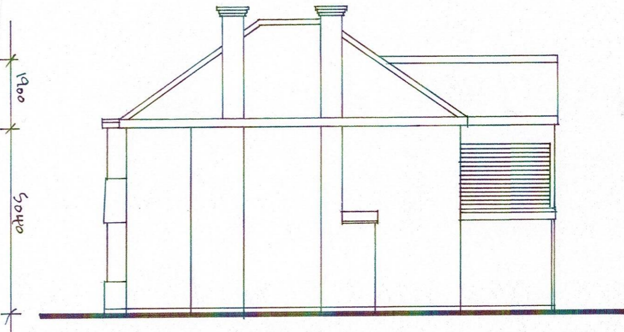
WEST ELEVATION.
