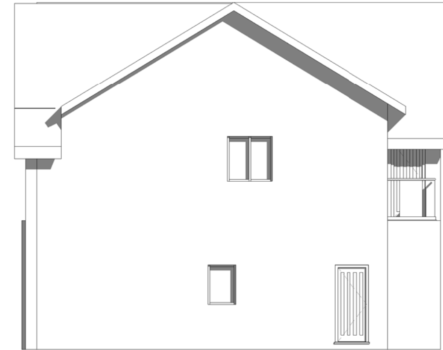
2 Right - Proposed 1 : 100
