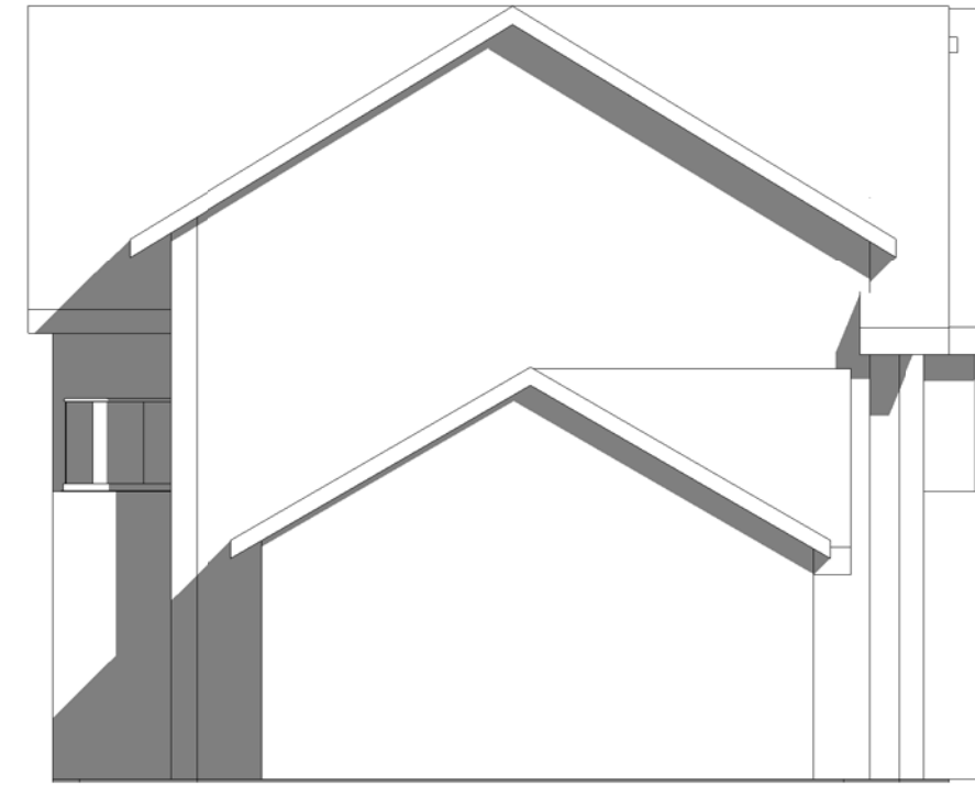
2 Left - Proposed 1 : 100
