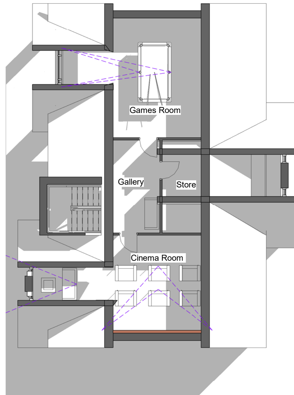
1 Level 2 - Proposed 1 : 100
