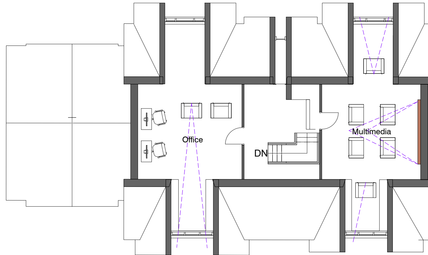
2 Level 2 - Proposed 1 : 100
