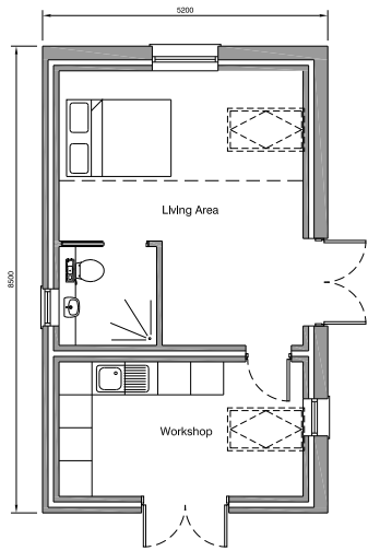
GF Plan
