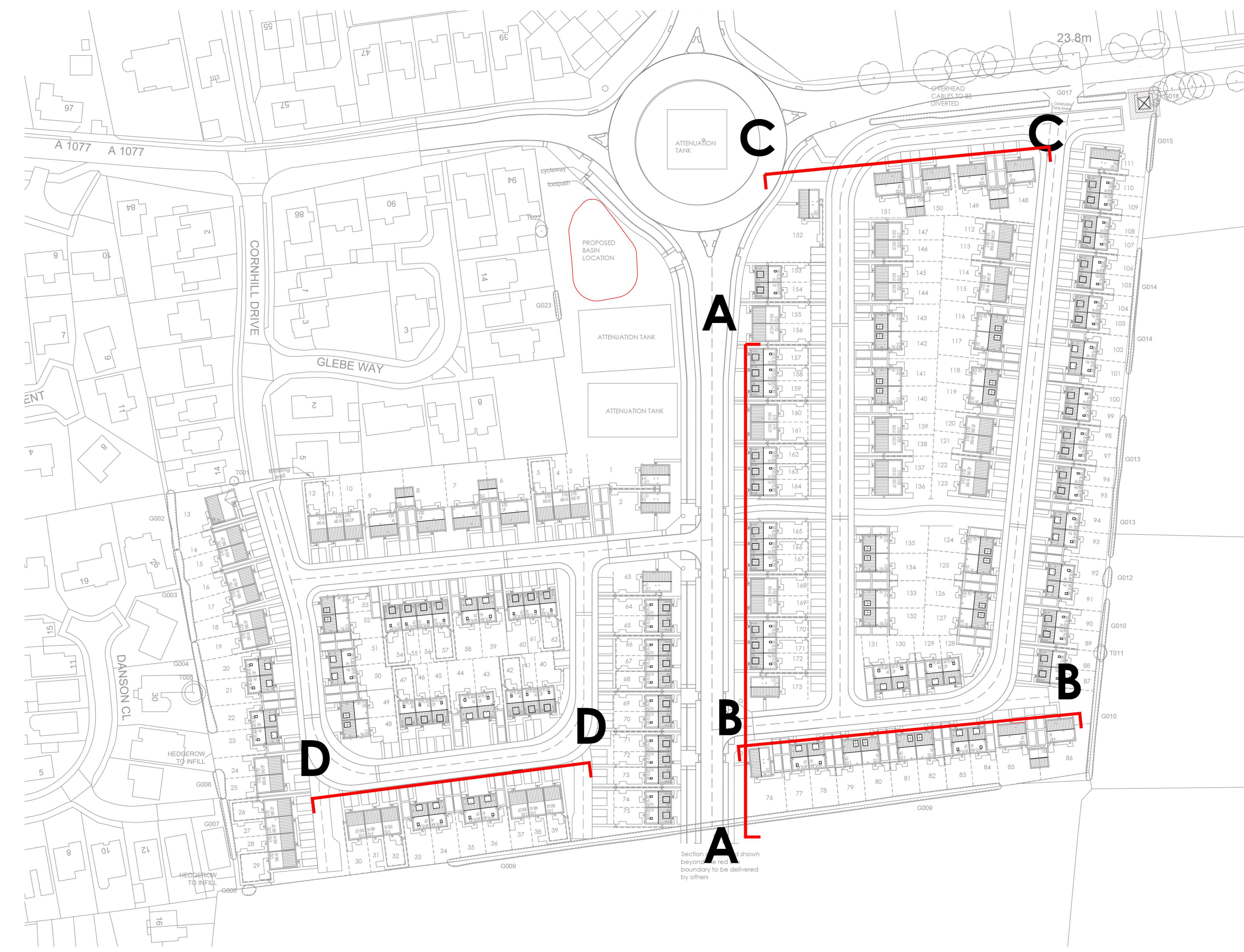
SITE LAYOUT @ 1:1000
