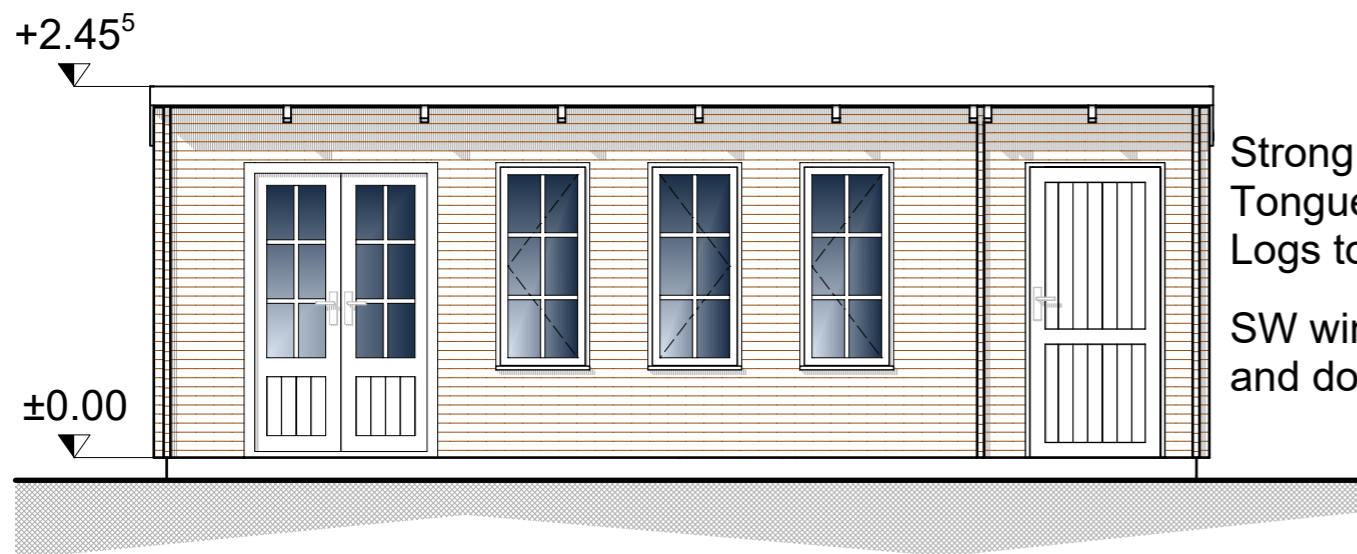
FRONT ELEVATION
