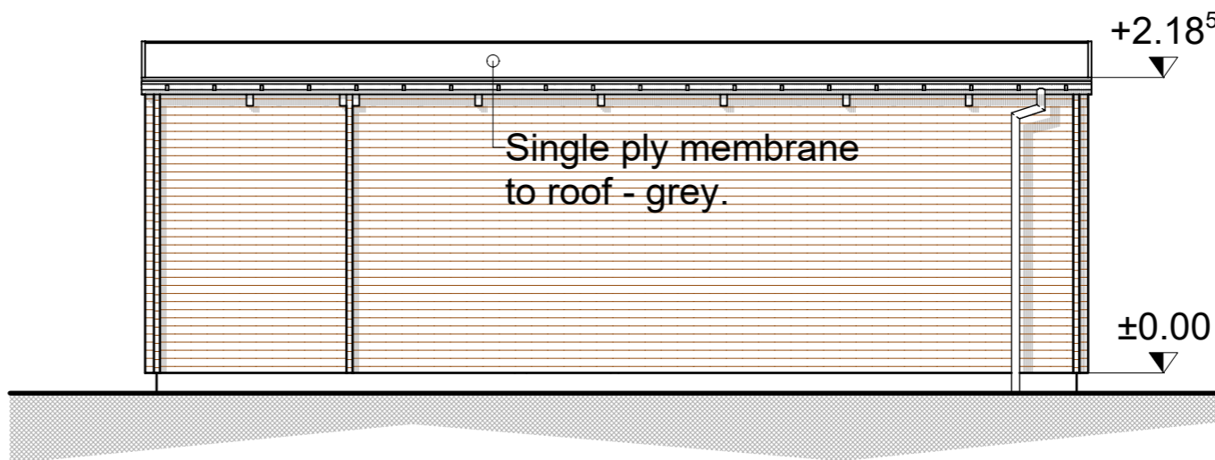
REAR ELEVATION
