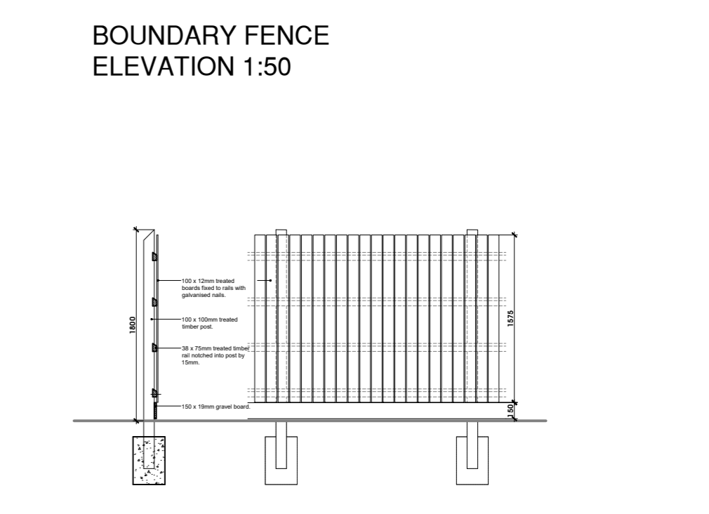
BIN AND CYCLE STORE CLOSE BOARDED TIMBER FENCE SECTION AND ELEVATION 1:50
