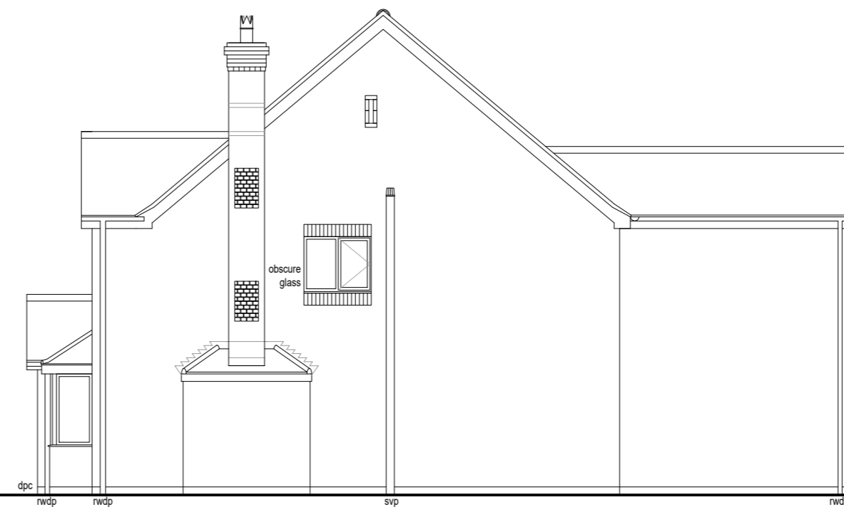
SIDE ELEVATION
