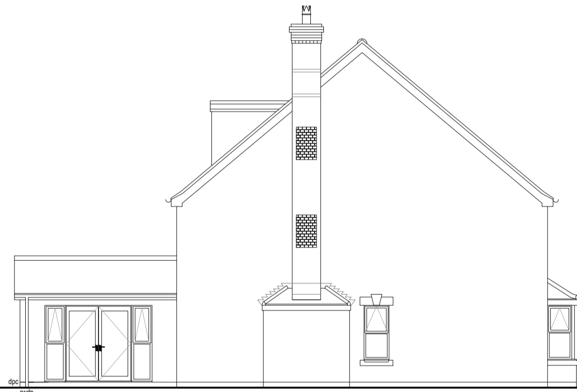
SIDE ELEVATION
