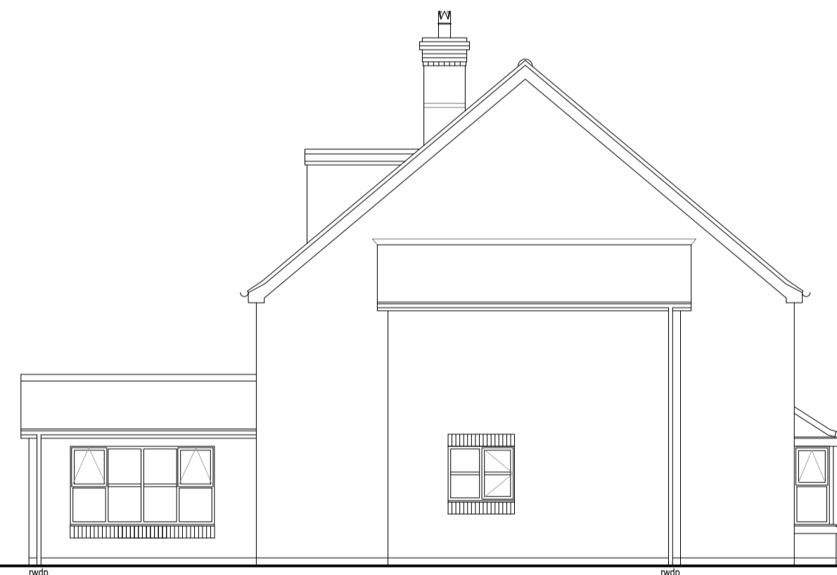
SIDE ELEVATION
