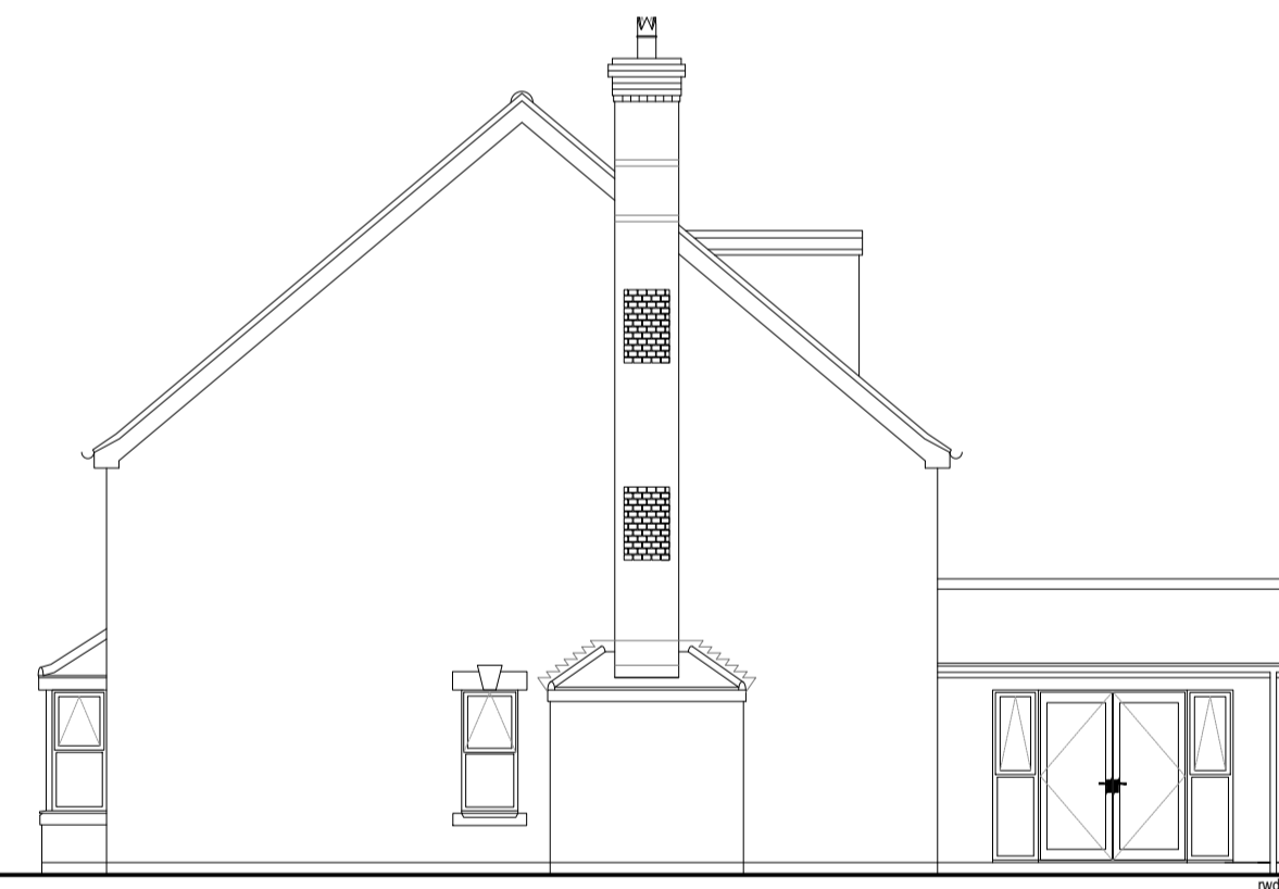
SIDE ELEVATION
