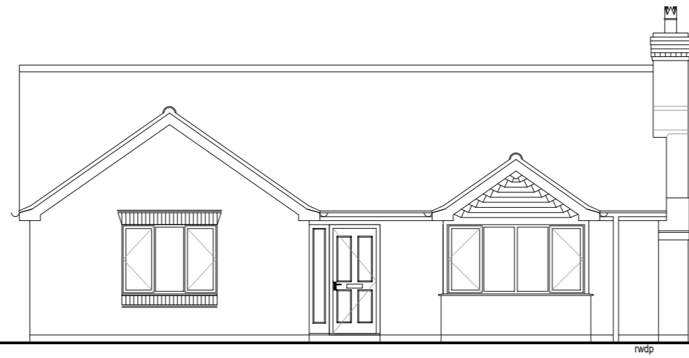
FRONT ELEVATION
