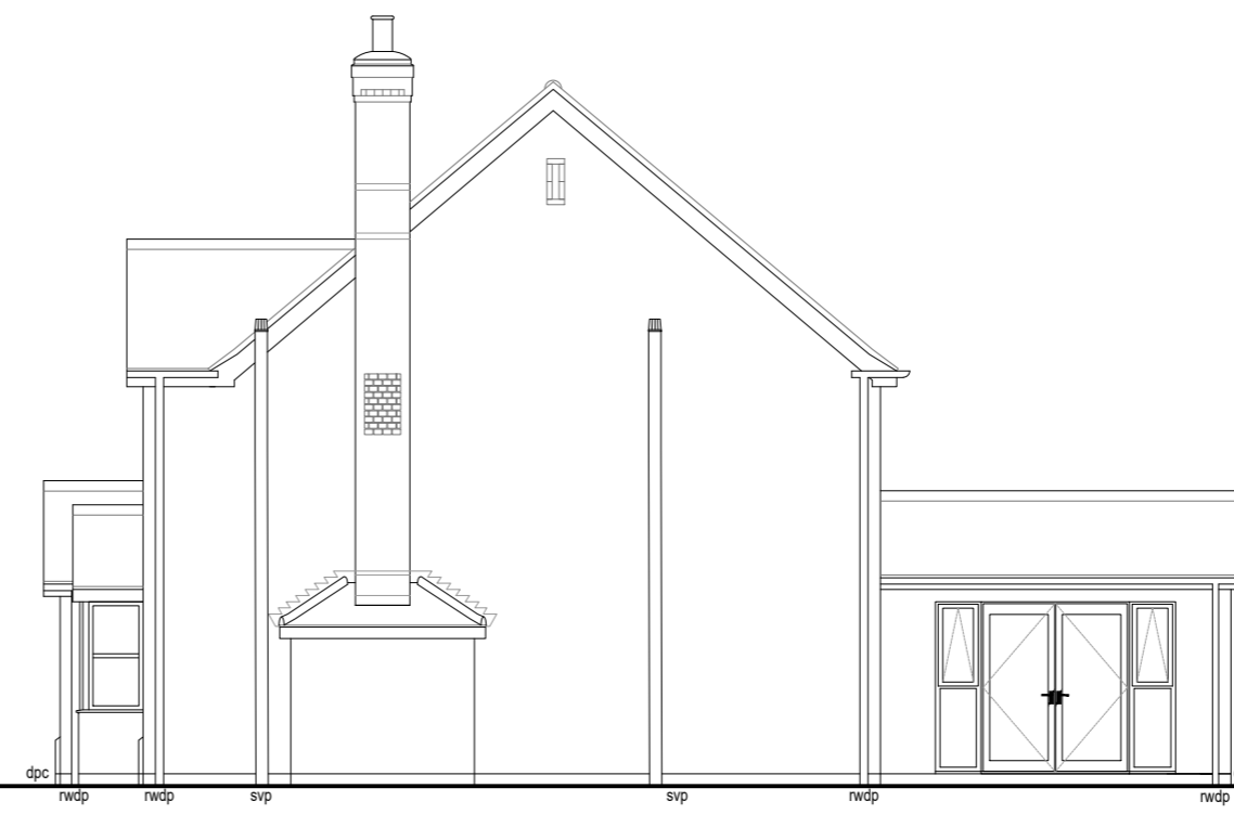
SIDE ELEVATION
