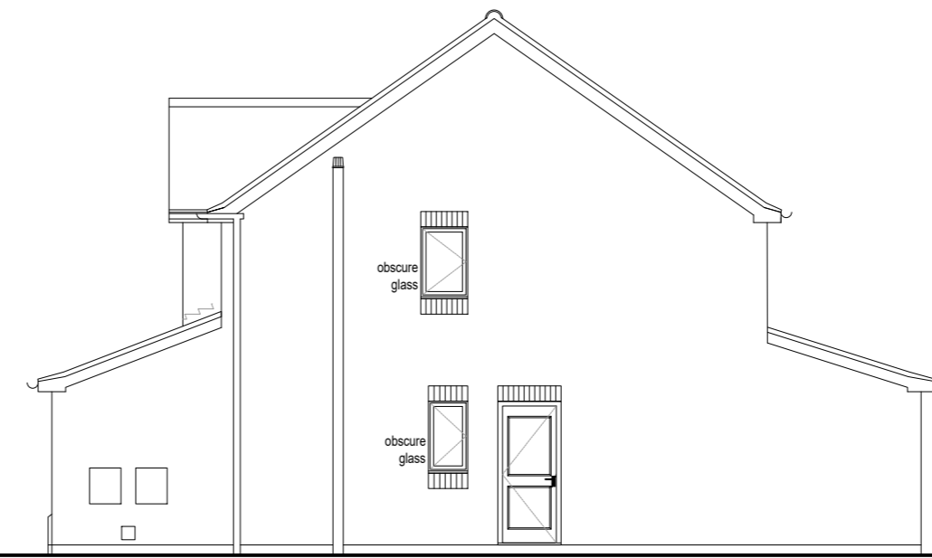
SIDE ELEVATION
