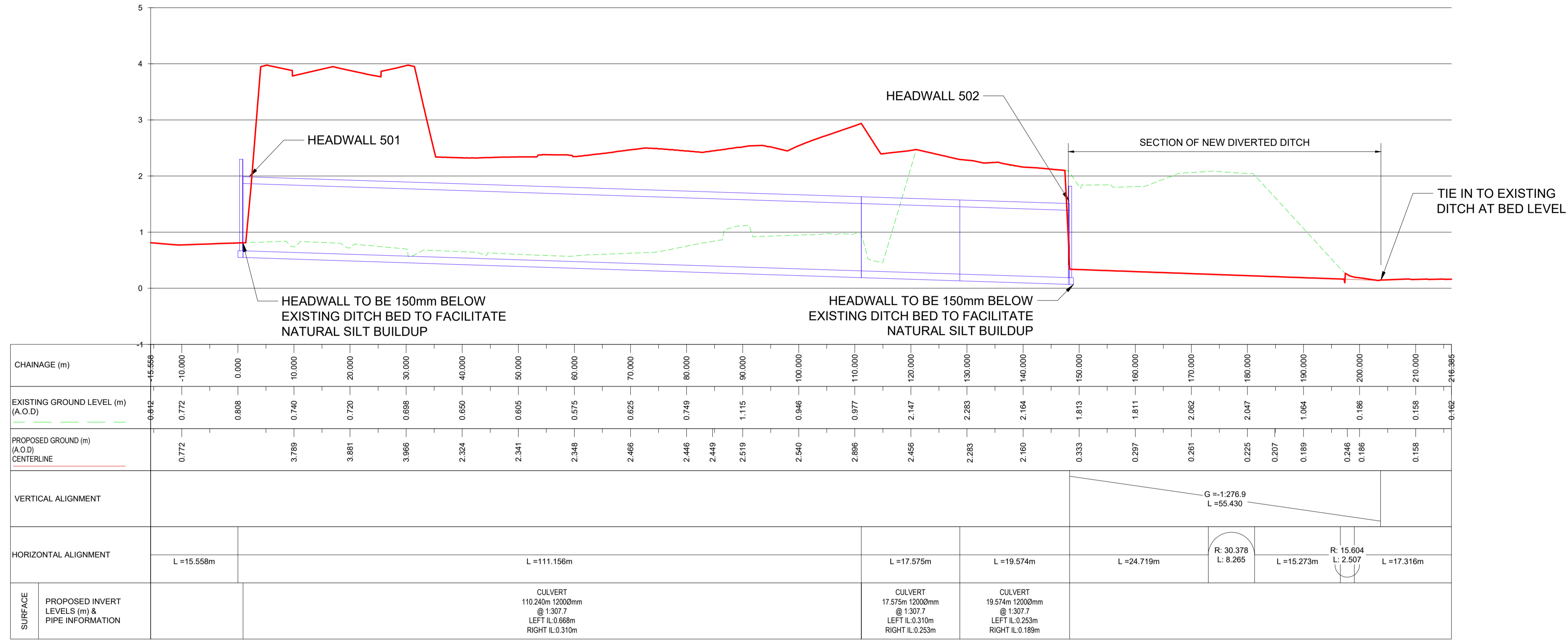
SOUTHERN DITCH DIVERSION - LONGSECTION SCALE: H 1:500, V 1:50. DATUM: -1.000
