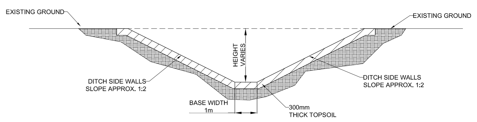
PROPOSED DIVERTED DITCH TYPICAL CROSS SECTION SCALE 1:100@A1
