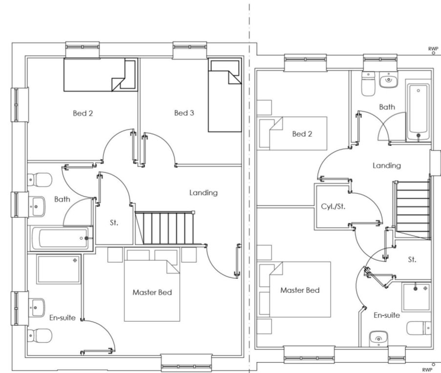
FIRST FLOOR
