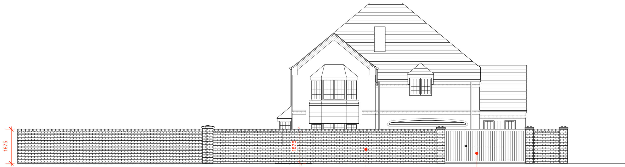
PROPOSED EAST BOUNDARY ELEVATION 1:100
